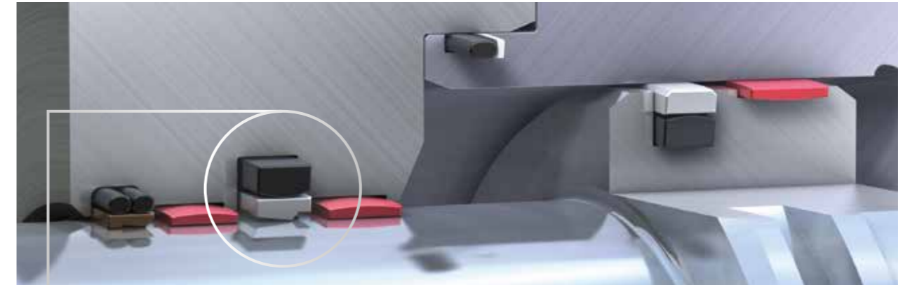
▲ Merkel Omegat OMS-S (rod) and Merkel Omegat OMK-S at the piston in combination with a Merkel PT 1 wiper and Merkel Guivex guide bands
