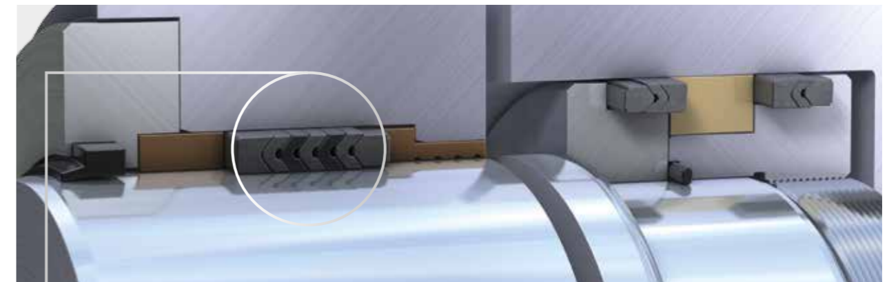
▲ Merkel V-packing set EKV at the piston and ESV at the rod combined with a Merkel P 6 wiper and metallic guide elements
